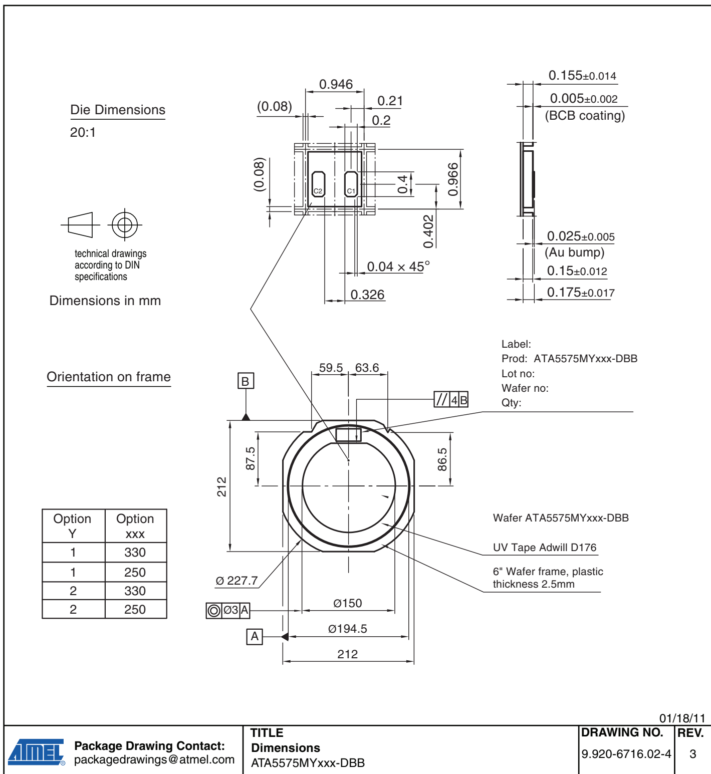
Figure 11-2. 6" Wafer on Foil with Ring and Gold Bumps 25µm
